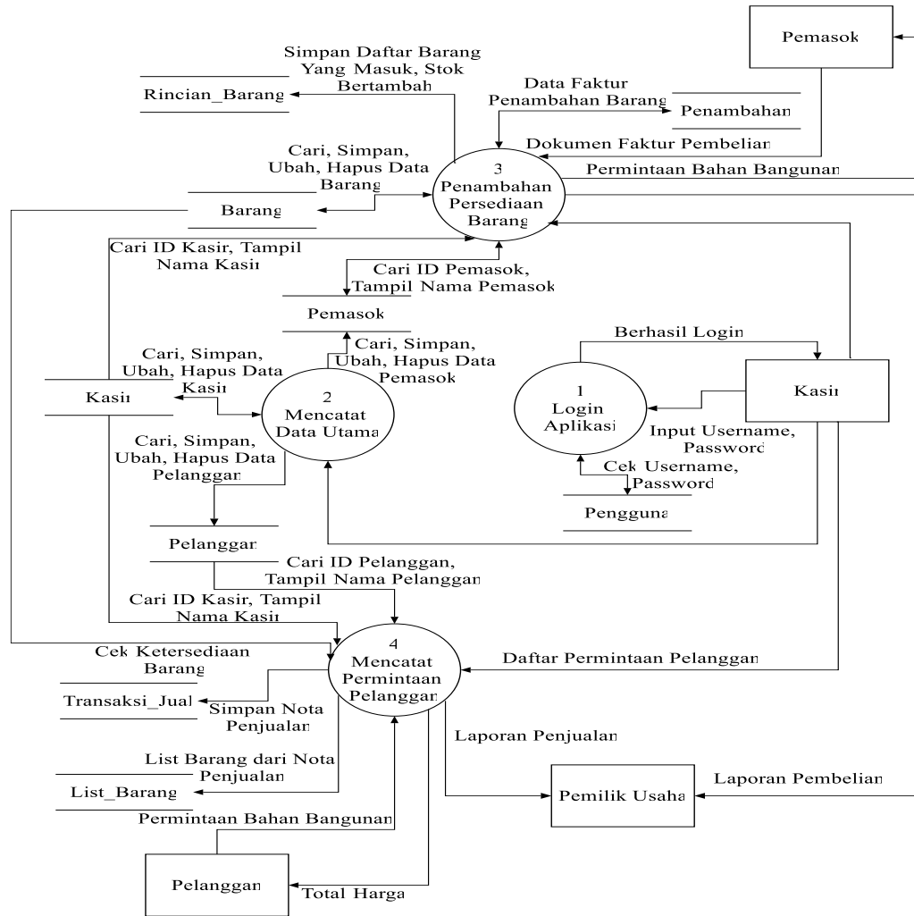
Gambar 2. DFD level 0
